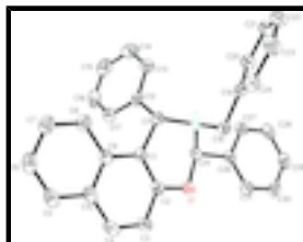
Fig. 1. The molecular structure of the title compound, showing the atom-numbering scheme. Displacement ellipsoids are drawn at the 30% probability level. H atoms are omitted for clarity.
